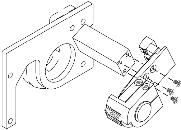
LED assembly
