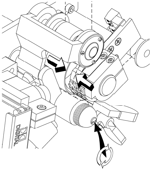
Adjust the lateral guide roller
