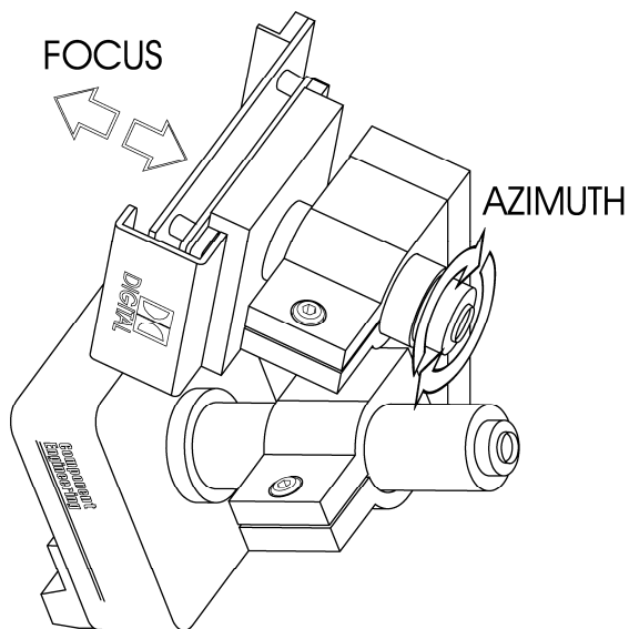
Adjust focus and azimuth of digital optics
