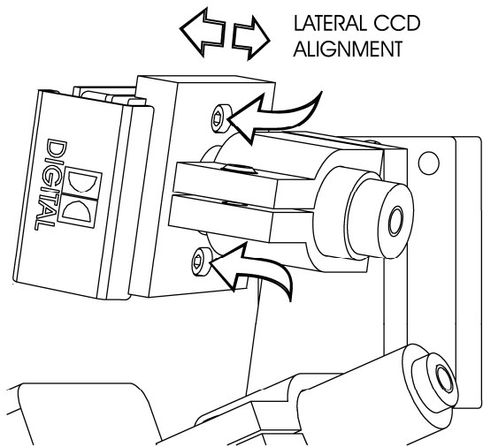
CCD board lateral adjustment
