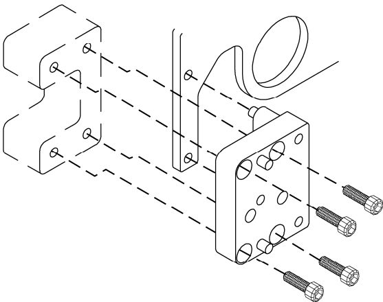
Install the adaptor block
