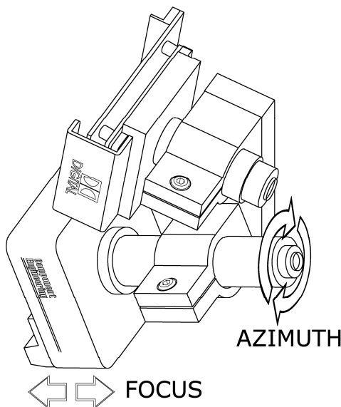
Analog focus and azimuth alignment
