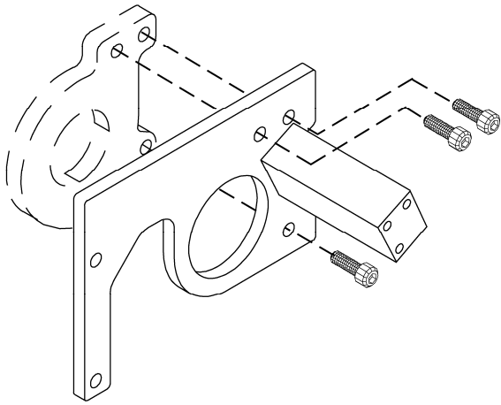
Position the locator plate
